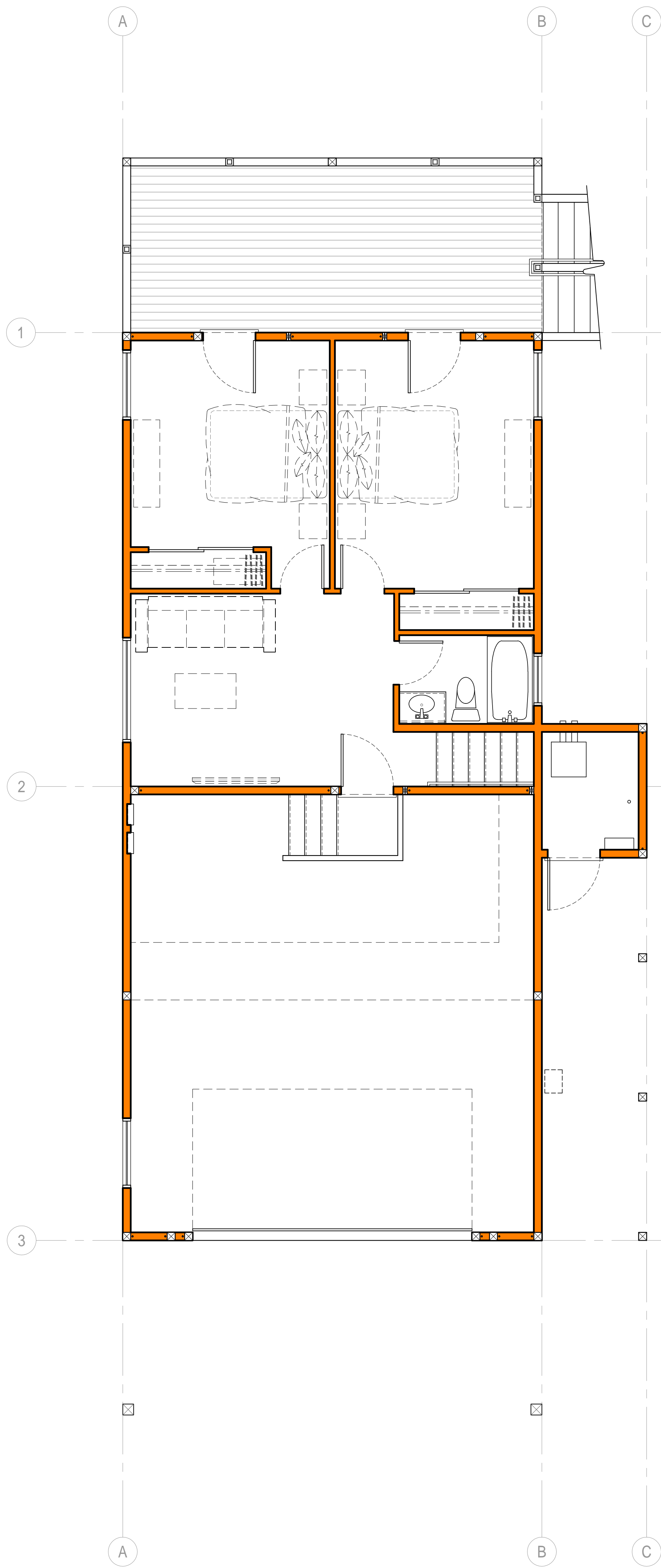
LF LOWER FLOOR
